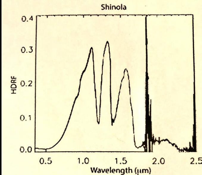
Figure 2a. Measurements of hemispherical-directional reflectance factor (HDRF) of Shinola. The solar zenith angle at time of acquisition was 33° with cloud-free skies.
